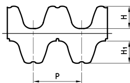
RTD5MDD - RTD8MDD
